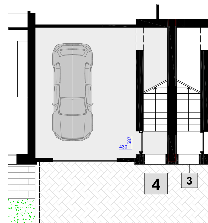
PIANO TERRA
