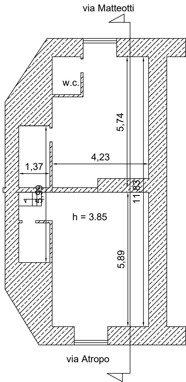
PLANIMETRIA PIANO TERRA
