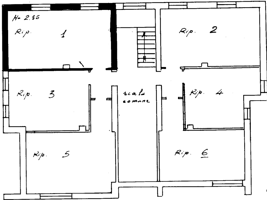
PIANO SEMINTERRATO
