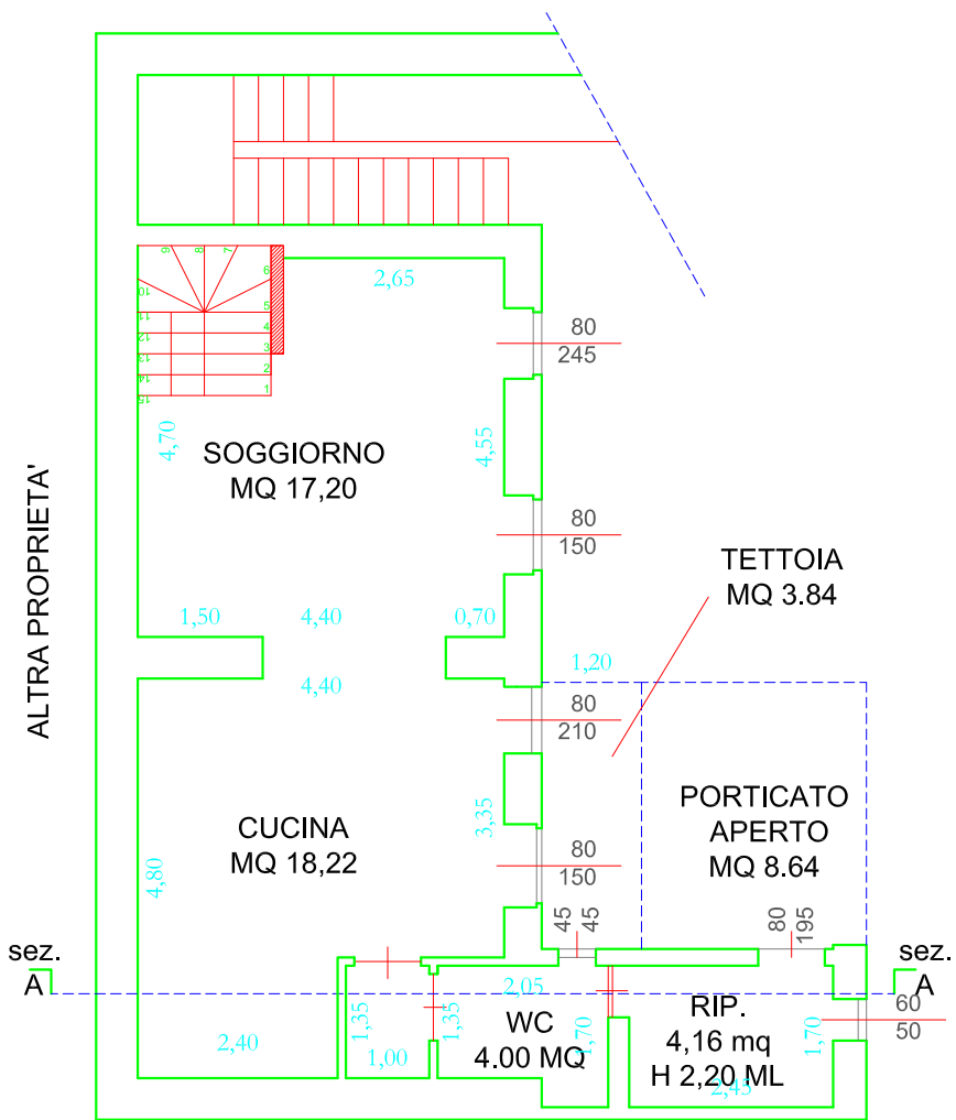
PIANTA PIANO TERRA H 2,70 ML
