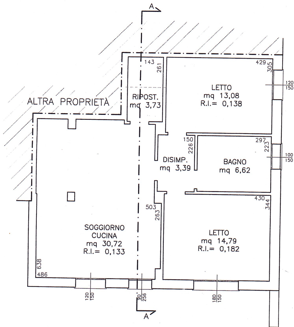
PIANO TERRA
