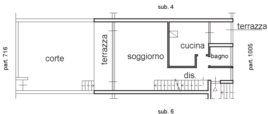
PIANO TERRA h=2.70
