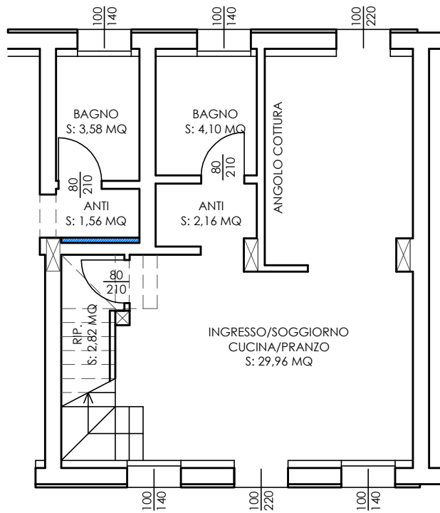
PIANO TERRA Scala 1:100
