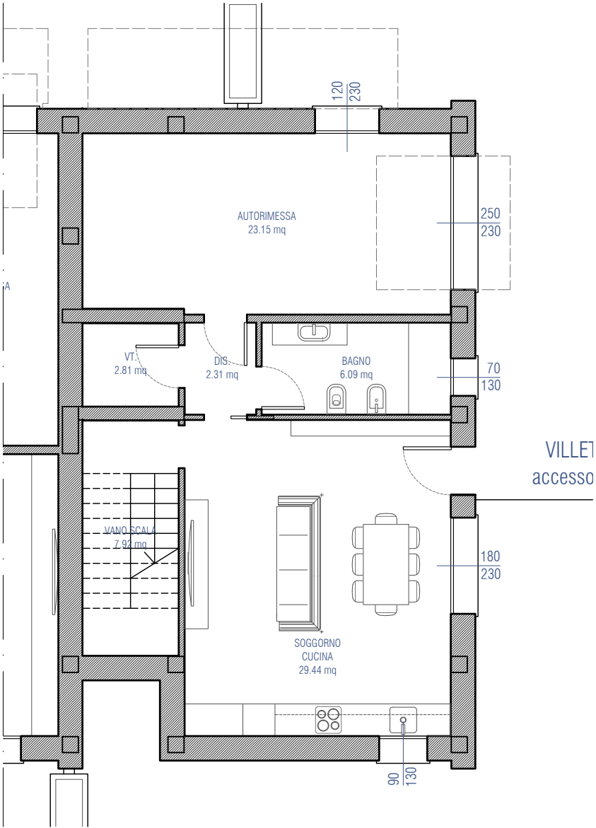
PIANO TERRA
