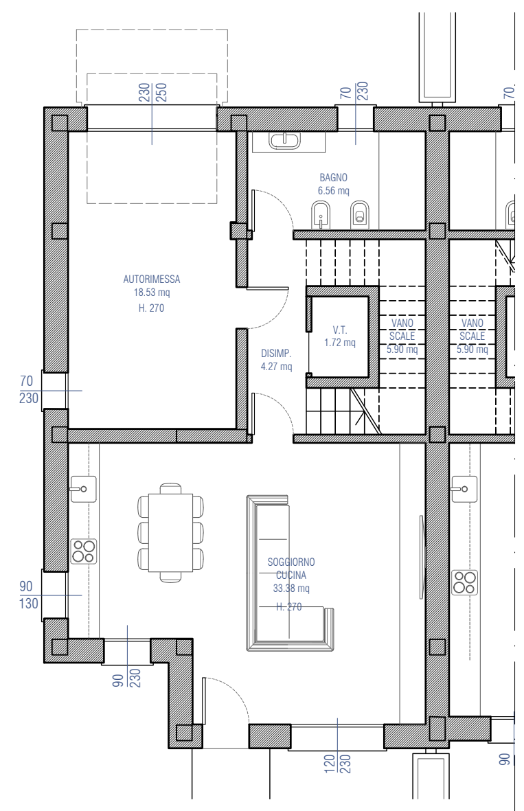
PIANO TERRA
