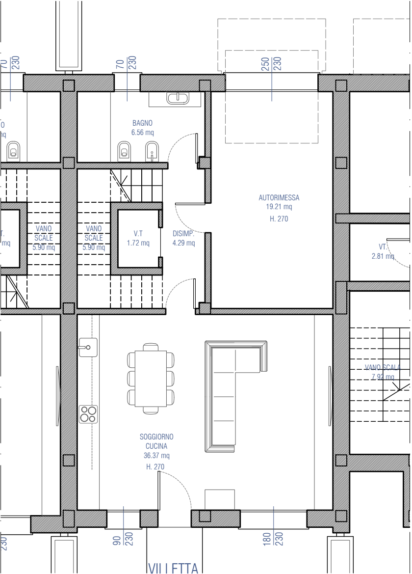
PIANO TERRA
