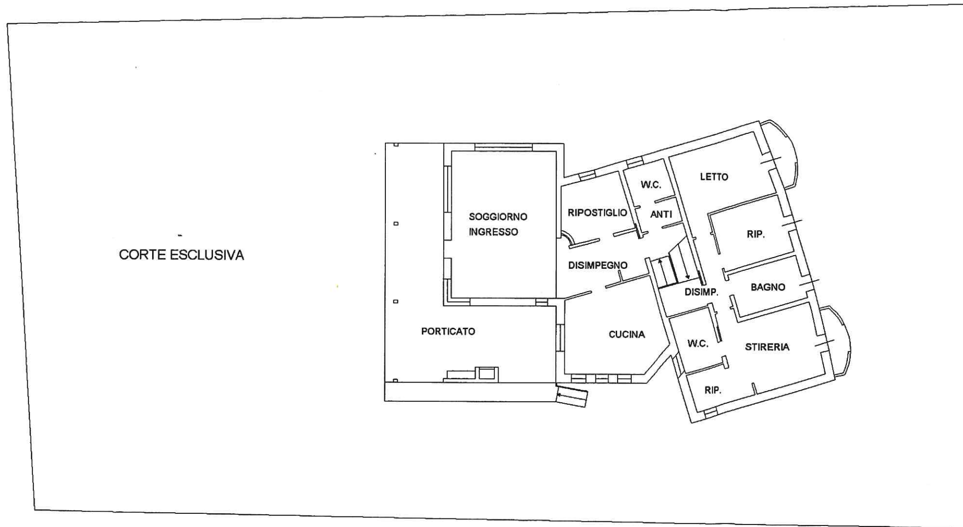
PIANO TERRA H=mt 2,70
