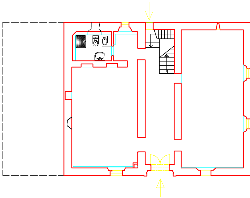
PIANO CANTINA
