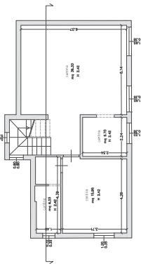
piano seminterrato
