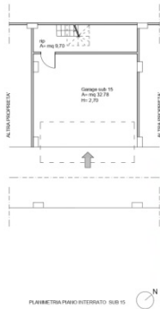
Planimetria garage sub 15
