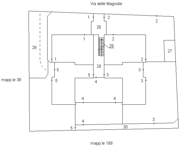
PIANO TERRA
