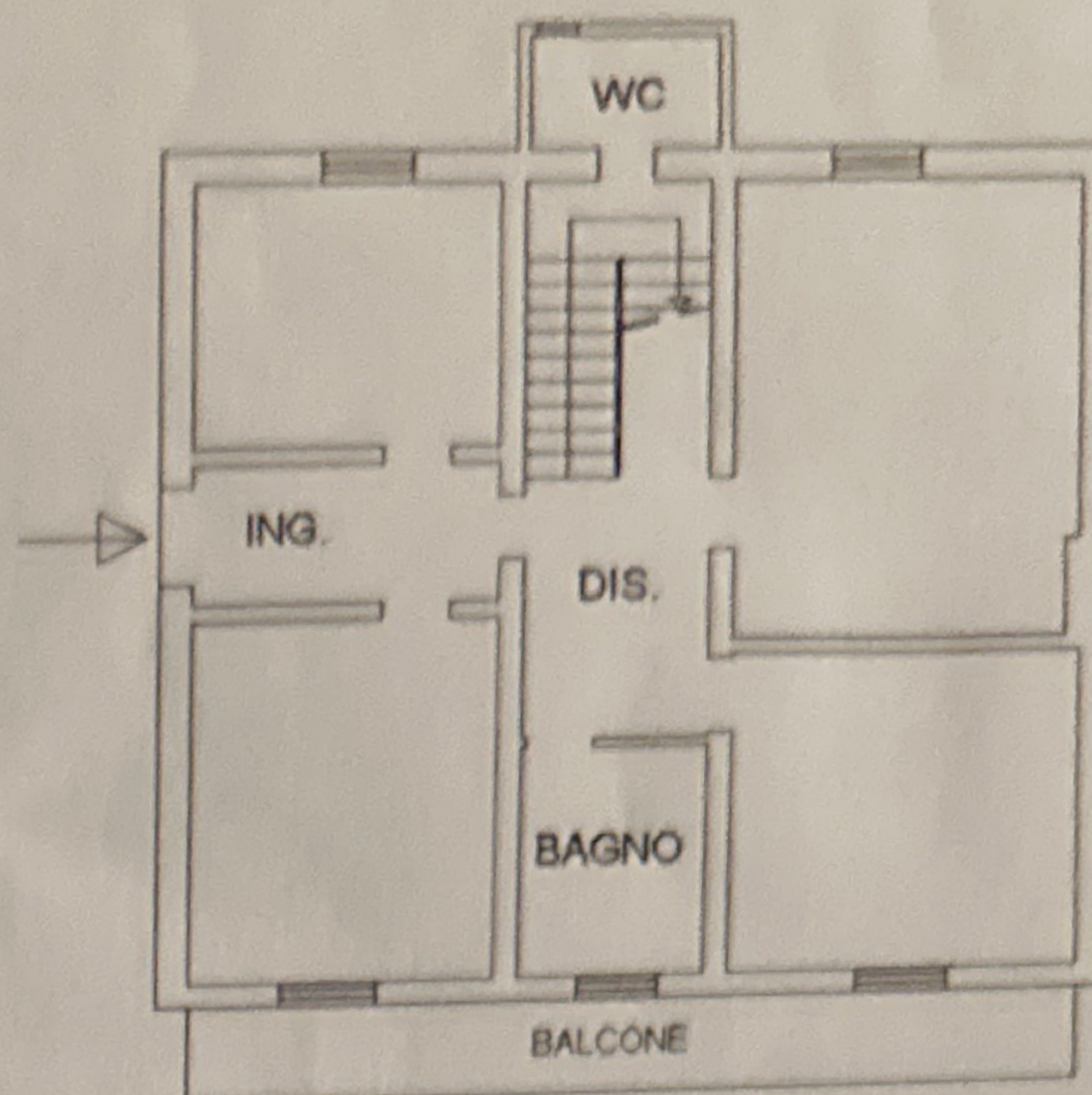
PIANO TERRA H= mt 2,80
