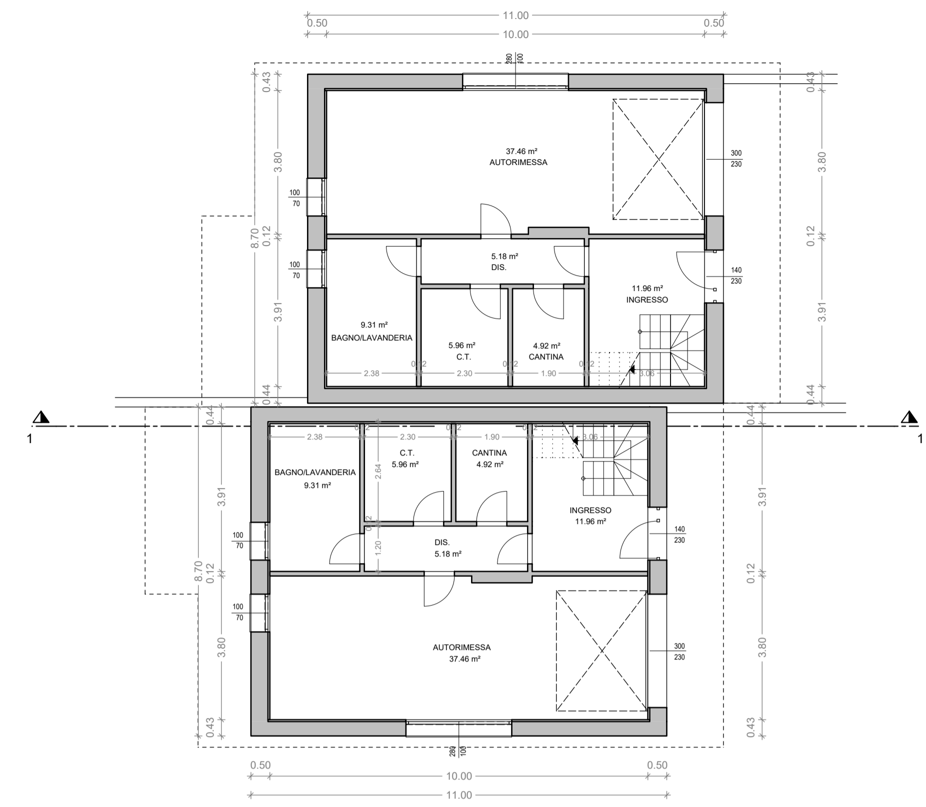
PIANO TERRA H=2.50 m
