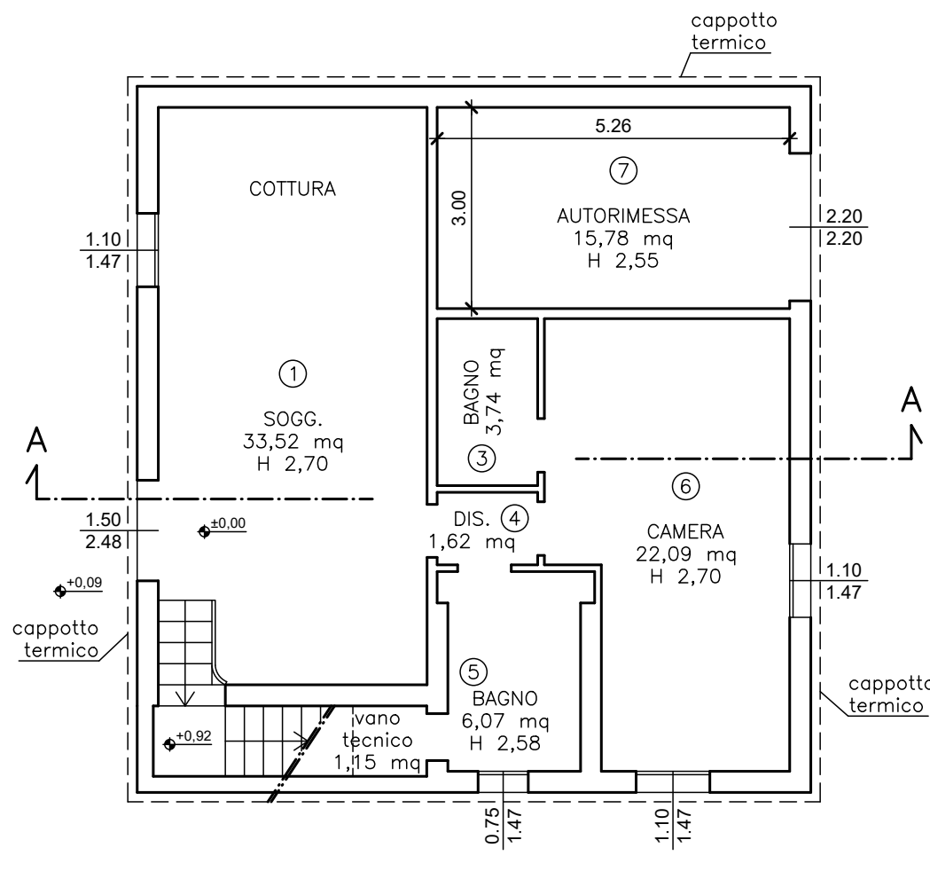
PIANO TERRA
