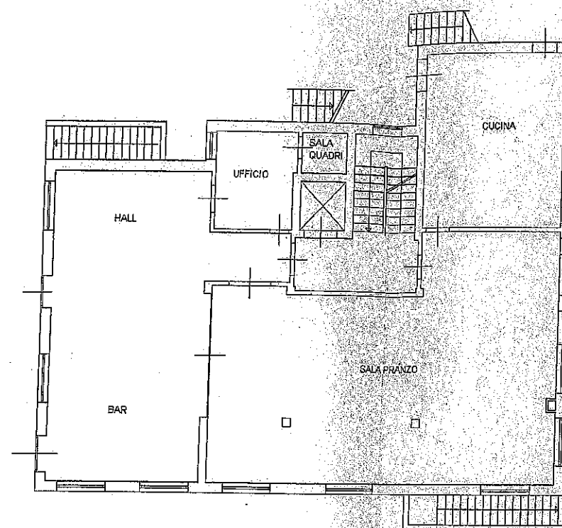
PIANO TERRA H= 2.80
