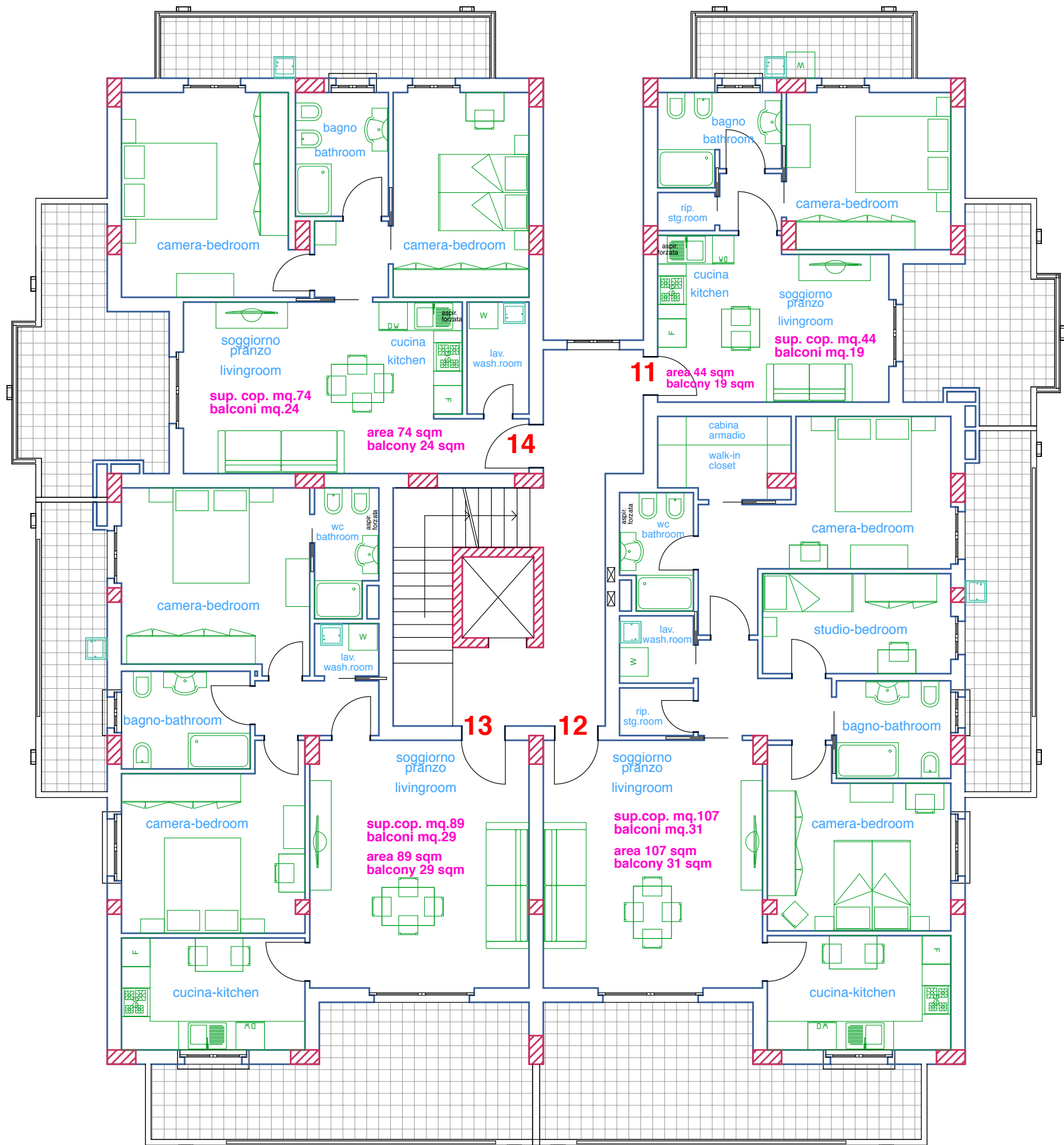
PIANO SECONDO SECOND FLOOR
