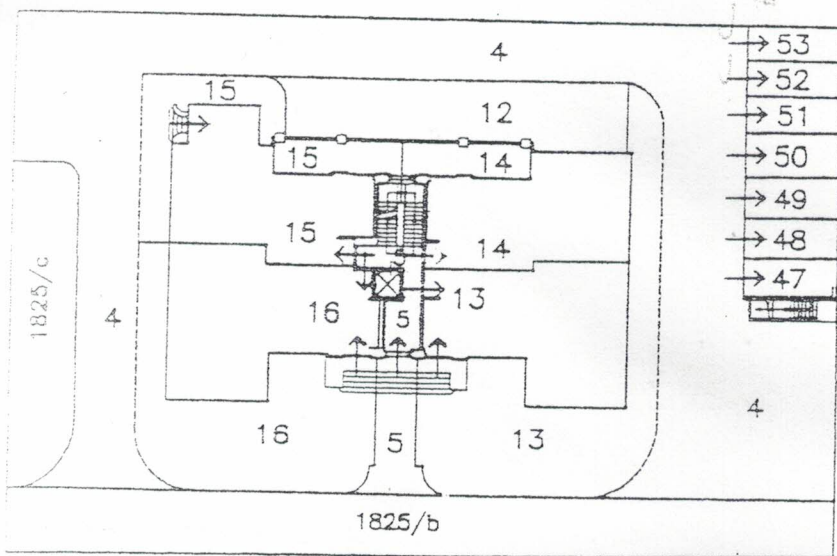
PIANO TERRA
